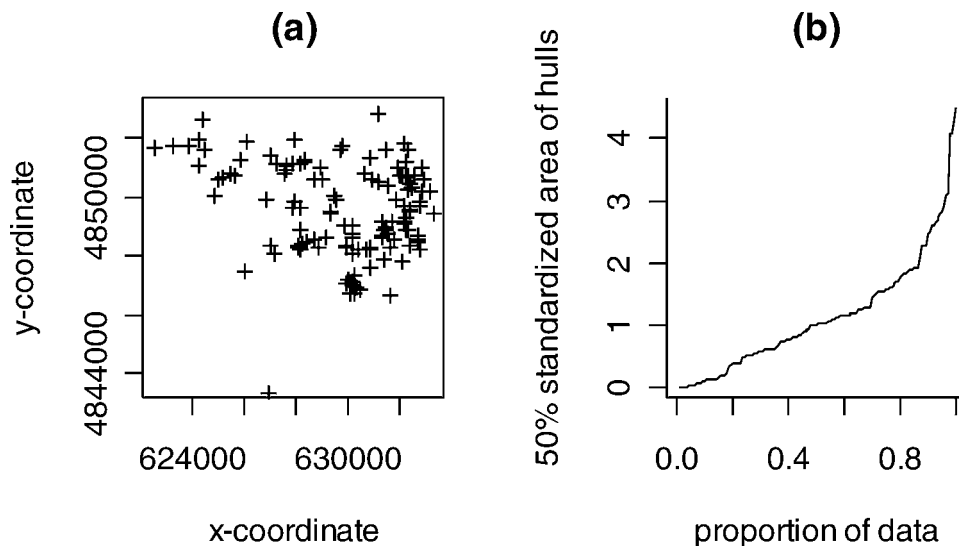
Figure 11. (a) Utilization distribution of elk data (Millsaugh 1999), (b) UD curve.
